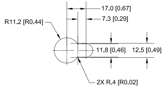
DETAIL A 2X THRU
